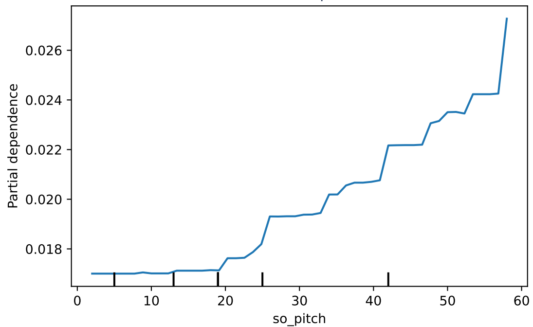
PDP — SO (pitch)
