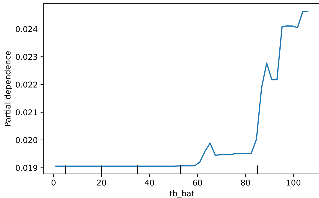
PDP — TB (bat)
