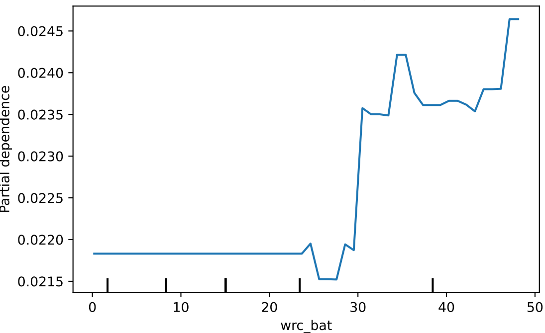
PDP — wRC (bat)
